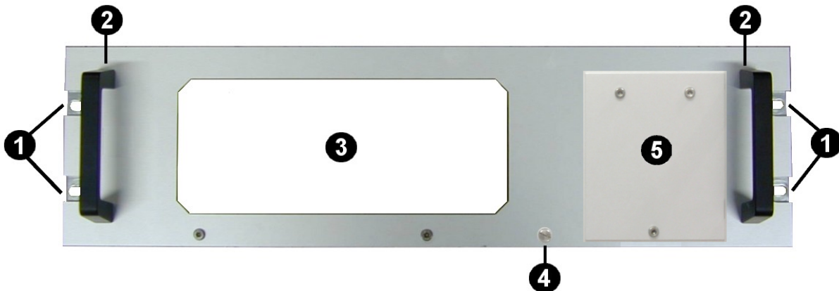
Fig. 12-1 Front view
