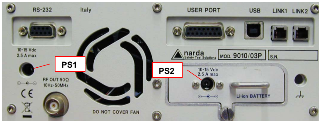
Fig. 9-2 Rear Panel
