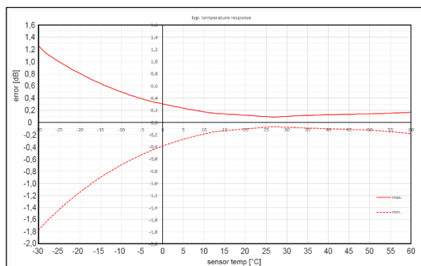
Fig. 1. Typical teperature response EFD-0392
