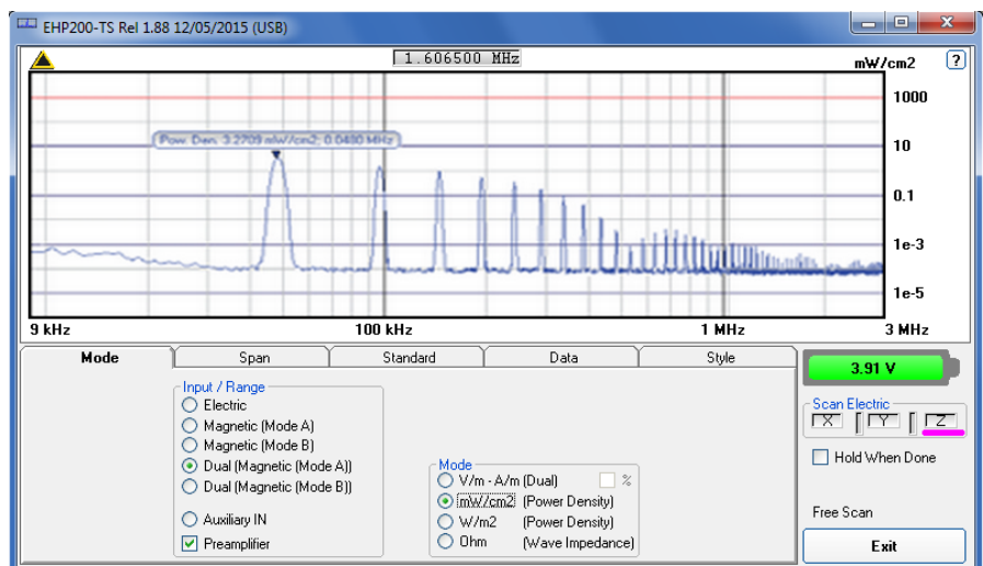
Fig.4-9 Power density spectrum is calculated over real electric and magnetic field measurement and therefore applicable to both far and near field conditions.
