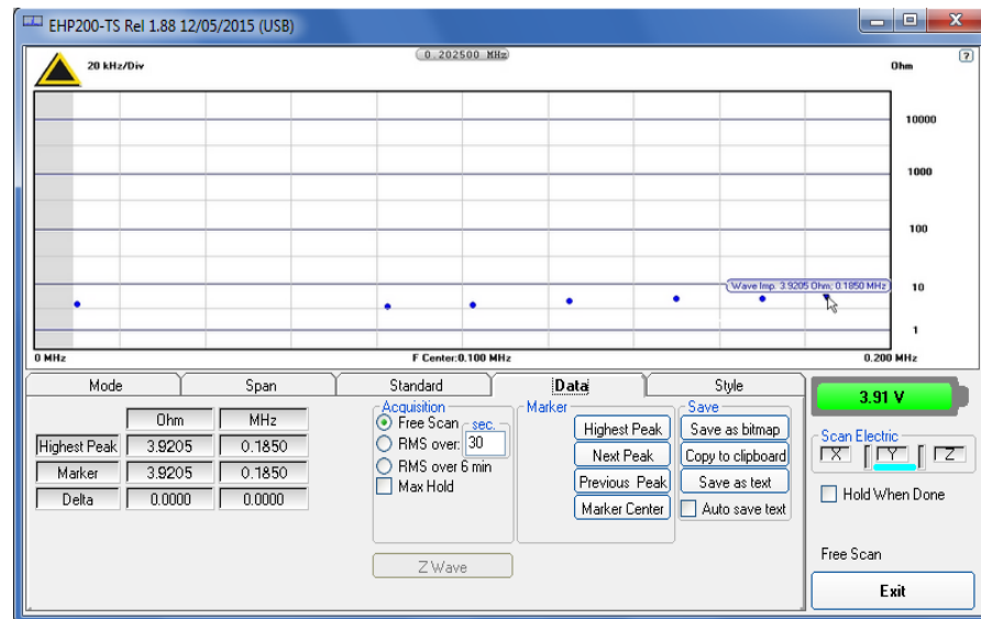
Fig.4-10 New wave impedance function
