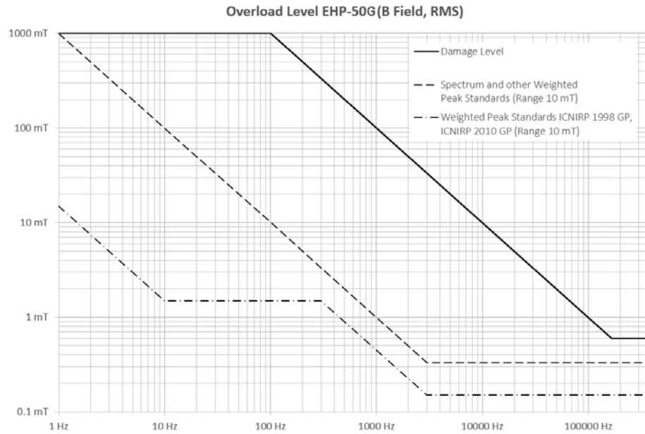
Fig. 1-4 Overload level EHP-50G (B Field, RMS)
