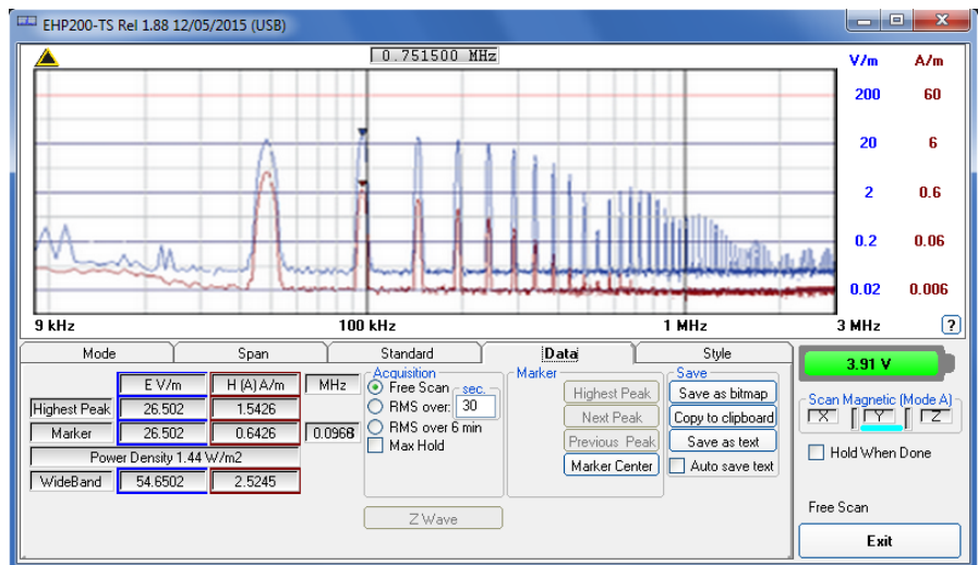
Fig.4-8 Both electric and magnetic fields can be displayed on the same graph.
