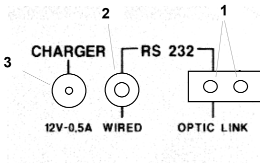
Fig. 9-7 Side panel
