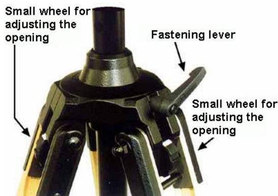
Fig. 9-8 TR-02A Tripod
