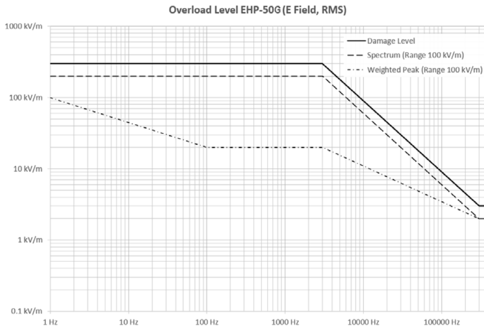
Fig. 1-5 Overload level EHP-50G (E Field, RMS)
